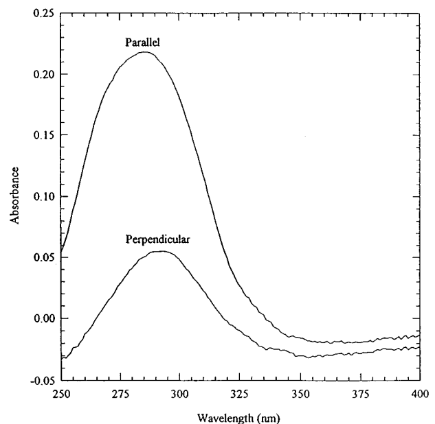
FIG. 1. Parallel and perpendicular absorbance spectra of a thin E7 film.
